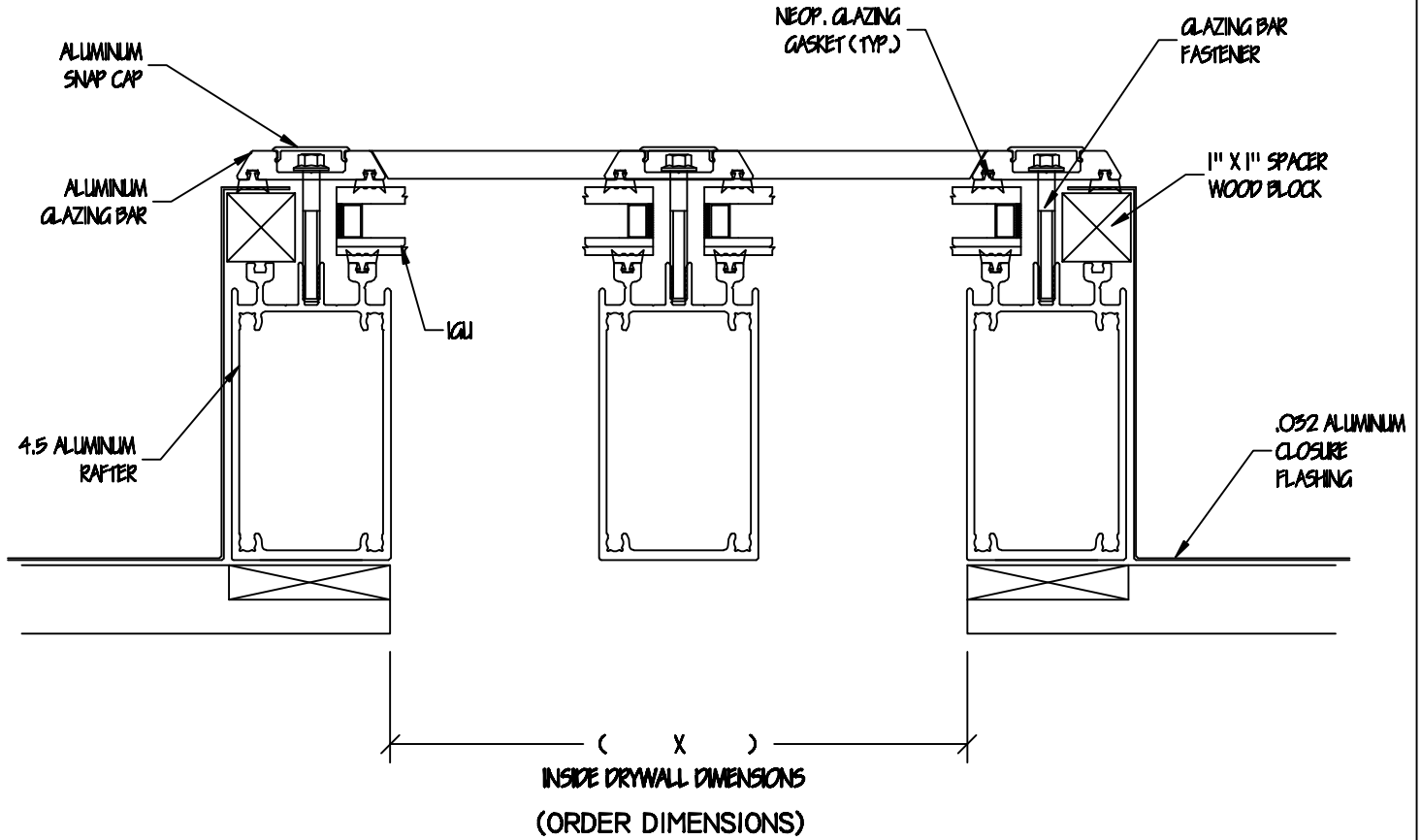
PLAN VIEW
